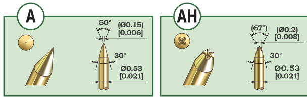
K2-0.72IIA-4.5M-4 Plunger Material: SK (Steel)
