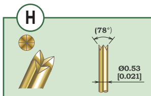
K2-0.72IIH-4.5M-4 Plunger Material: SK (Steel)
