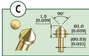
K2-0.72IIC-4M1.0-1 Plunger Material: SK (Steel)
