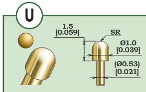
K2-0.72IIU-4.5M1.0-4 Plunger Material: SK (Steel)
