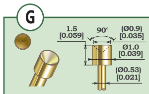
K2-0.72IIG-4.5M1.0-2 Plunger Material: SK (Steel)
