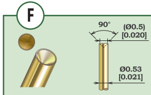
K2-0.72IIF-4.5M-5 Plunger Material: SK (Steel)
