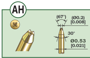
K2-0.72IIAH-4.5M-4 Plunger Material: SK (Steel)
