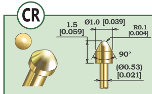
K2-0.72IICR-4.5M1.0-3 Plunger Material: SK (Steel)
