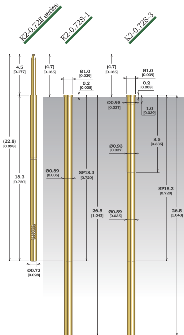
K2-0.72IIIC-4.5M1.0-4 Plunger Material: SK (Steel)
