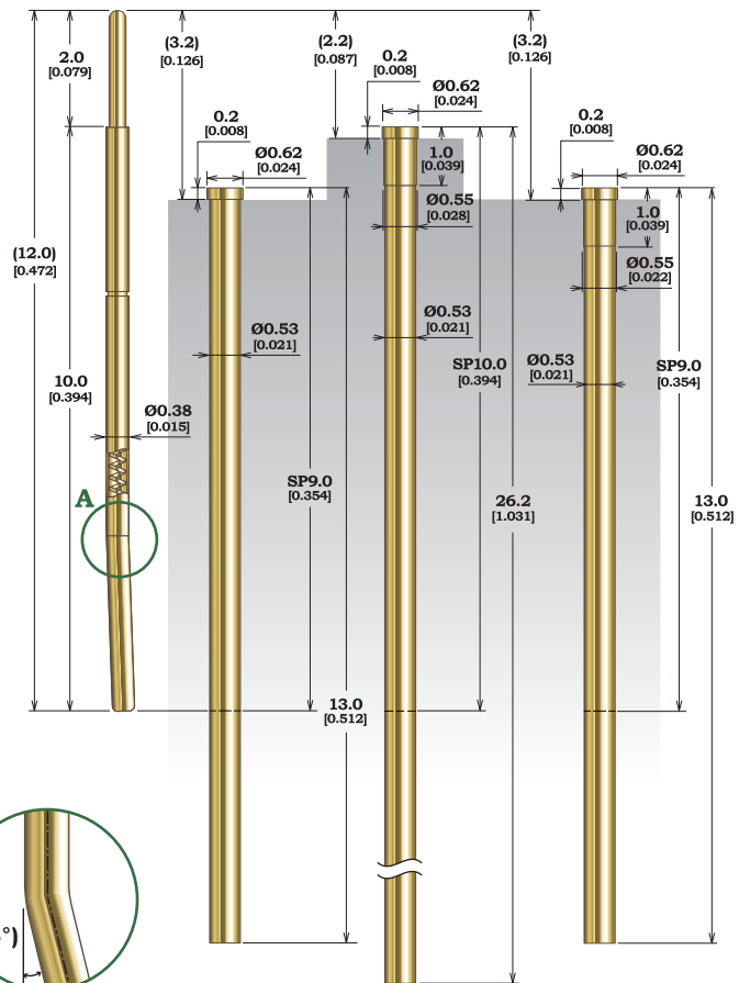
抜け止め用曲げ加工付 Bending for retention
